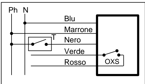
2 points control + 1 auxiliary switch KAM980L01.800 - KAM980L03.800
