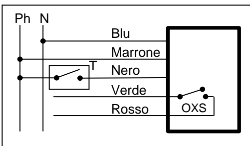
2 points control + 1 auxiliary switch KAM980L01.800 - KAM980L03.800
