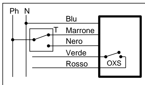
3 points control + 1 auxiliary switch KAM980L04.800 - KAM980L07.800
