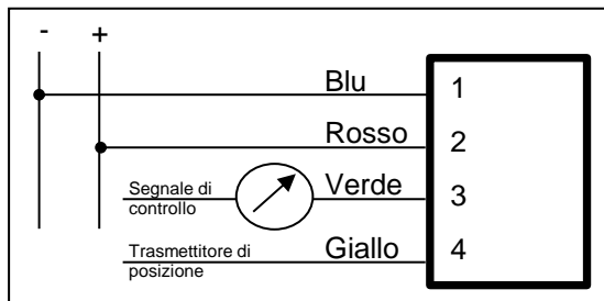
Control signal 0-10V KAM980L05.800
