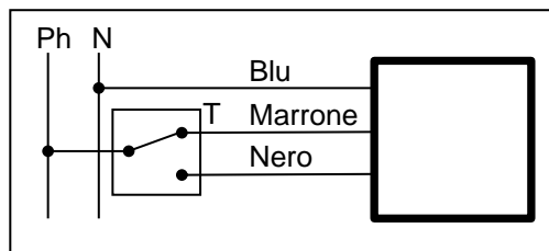
3 points control KAM980L06.800
