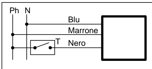
2 points control KAM980L00.800 - KAM980L02.800
