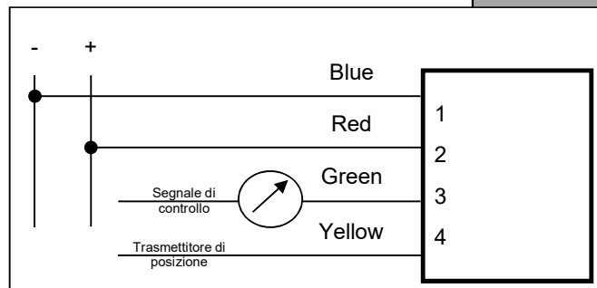
0 -10V control signal
