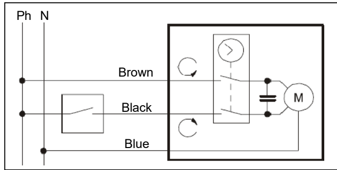
2 points control
