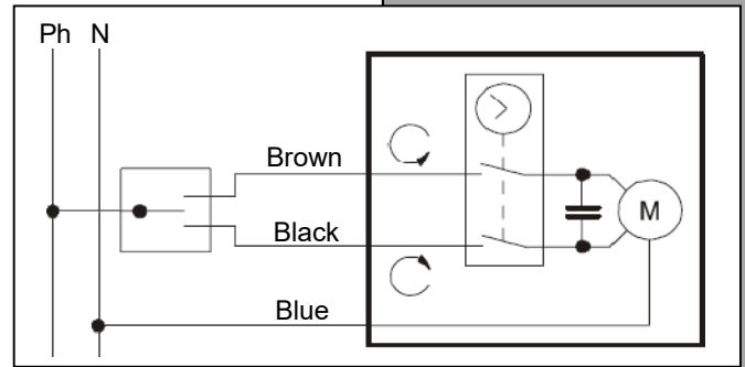
3 points control
